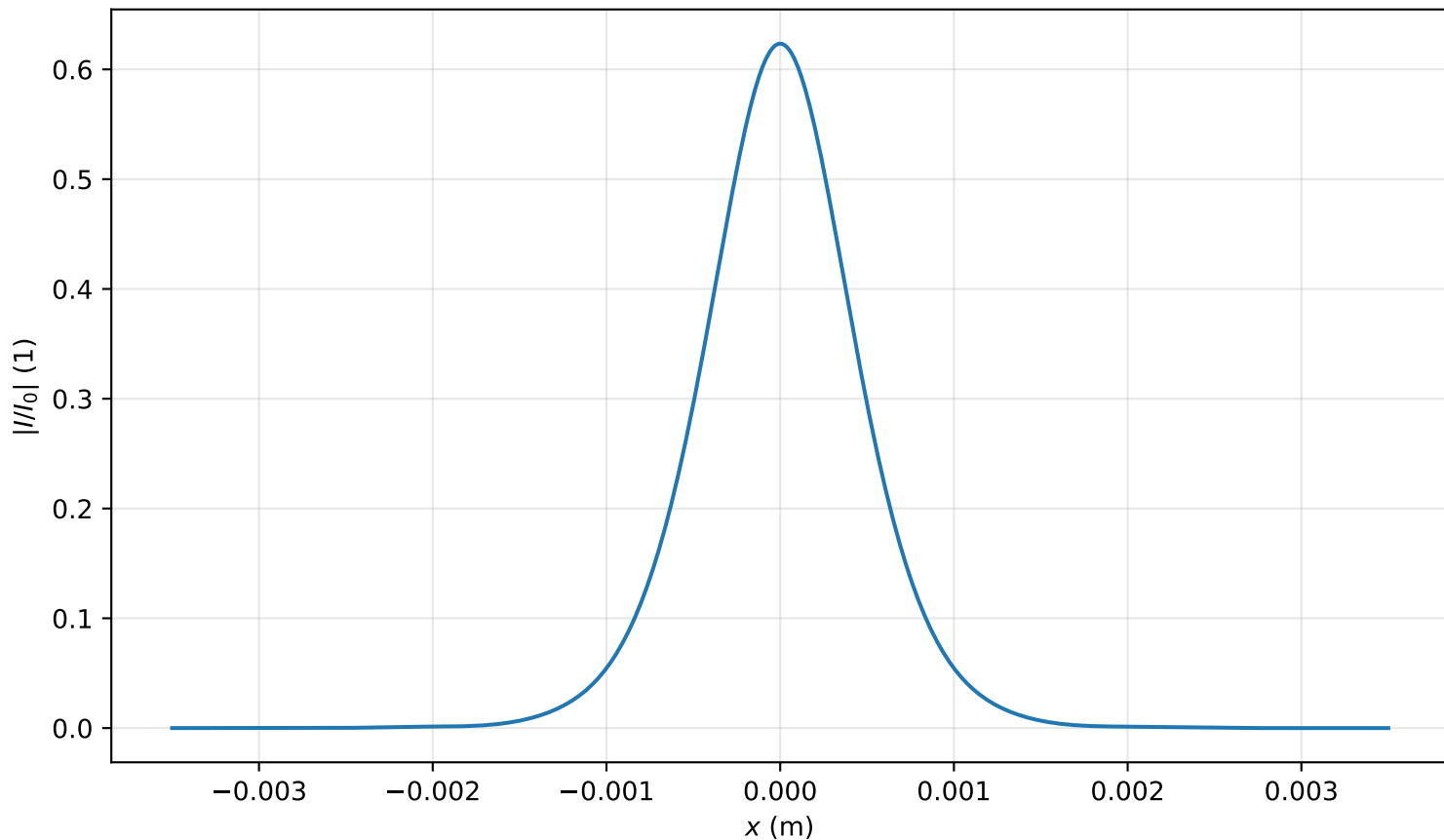
Intensity profile I(x, y = 0, z = 3.981m)/I_0 , P_{in}=0.7P_{cr} , artificial time
